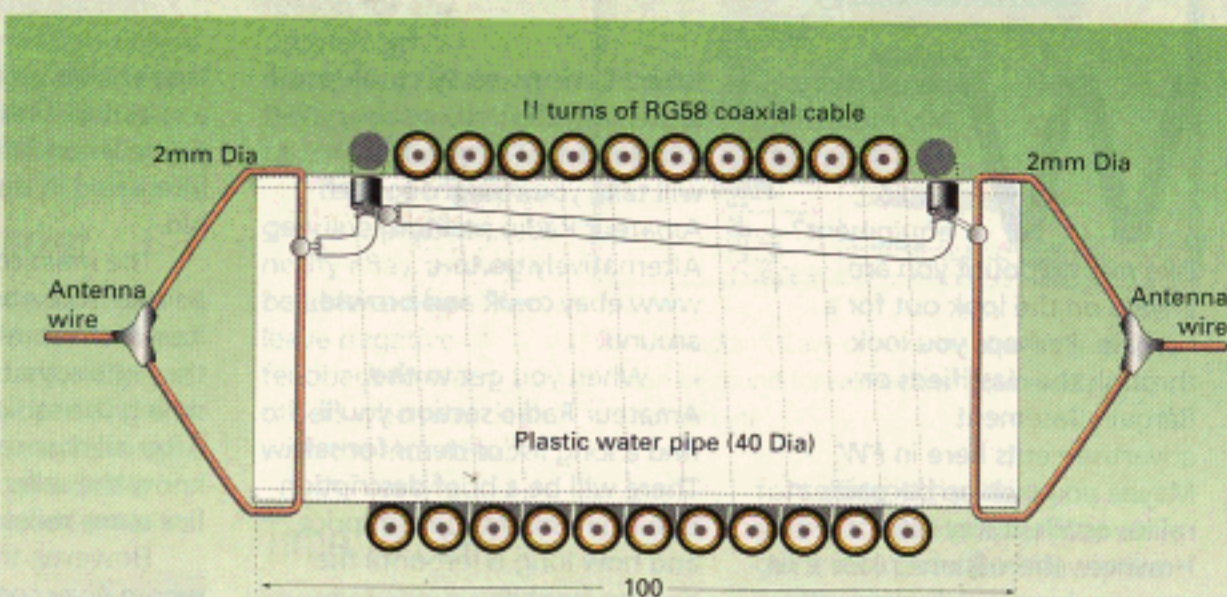
● Fig. 3: A cross-section of the 7MHz trap made from a length of 40mm diameter, plastic pipe and some RG58 coaxial cable. (See text for more detail).
