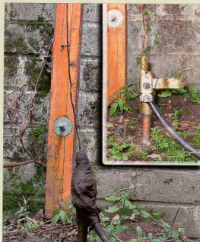
● Fig. 2: After the trimming adjustments, the bottom of the antenna is covered in a thick covering to waterproof the join. The join itself and the 'Tenby' clip are seen in the inset photograph.
